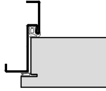
Stahl-Eckzarge
