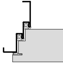
Stahl-Eckzarge
